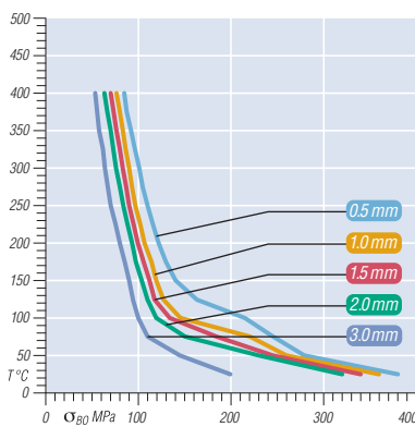
The diagram above shows this values for different gasket thicknesses.
